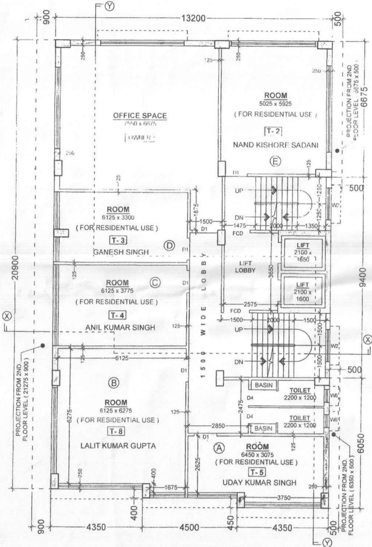
PROPOSED FIRST FLOOR PLAN. (REHABILITATED TO PARTLY TENANTS & PARTLY OWNERS)
