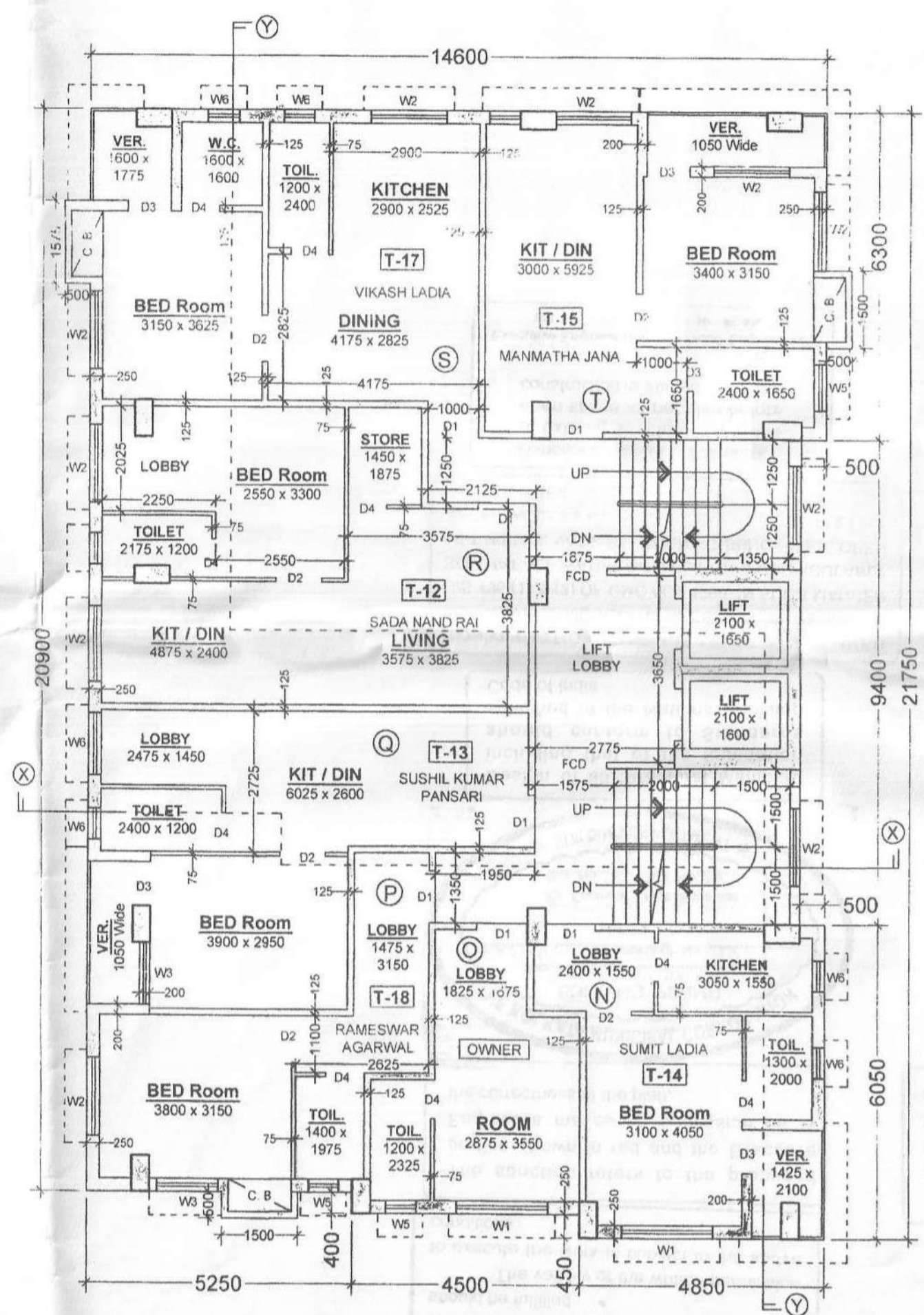
PROPOSED FIFTH FLOOR PLAN. (REHABILITATED TO THE EX. TENANTS)
