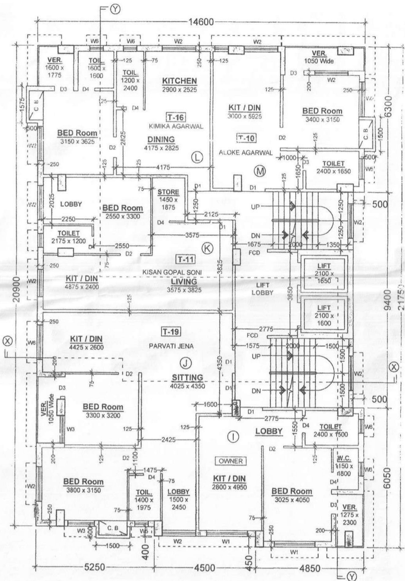
PROPOSED FOURTH FLOOR PLAN. (REHABILITATED TO PARTLY TENANTS & PARTLY OWNERS)
