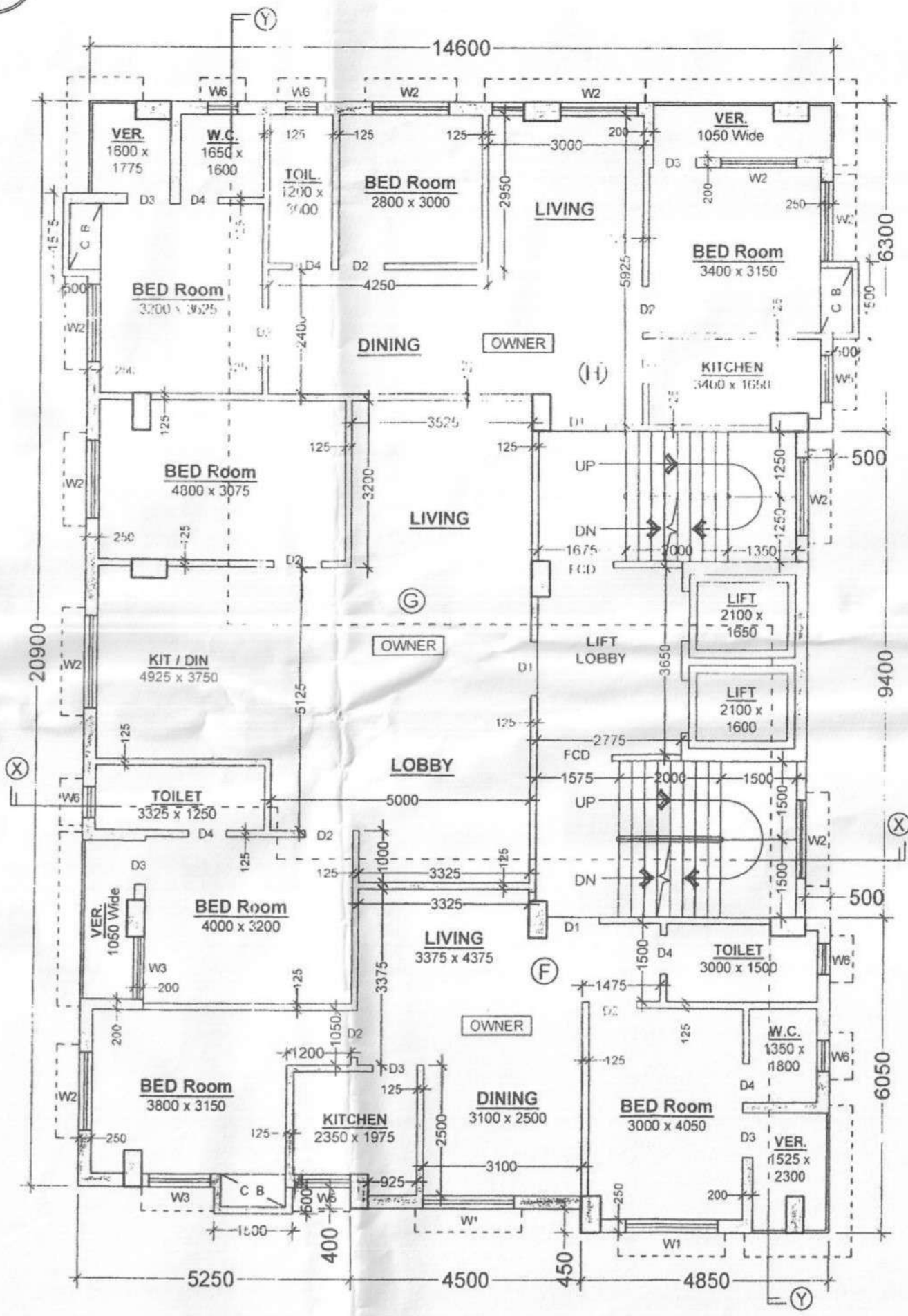
PROPOSED SECOND, THIRD & SIXTH FLOOR PLAN.
